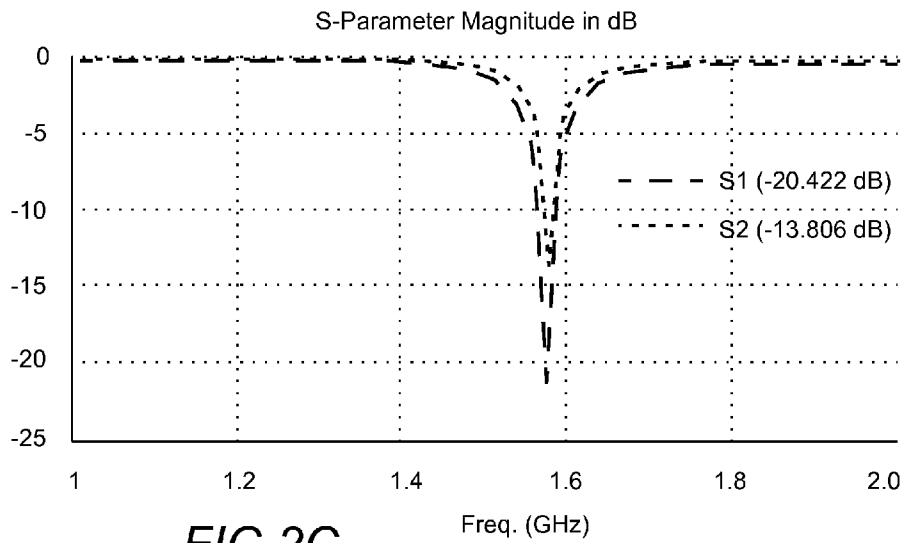
FIG.2C (Prior Art)
